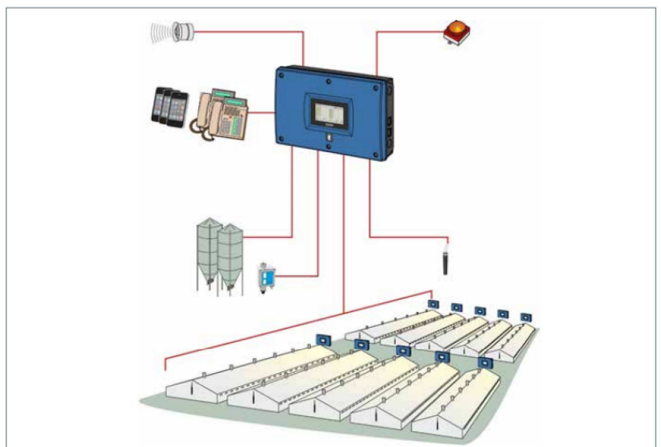
Multiple connection options with the DOL 2400 alarm system
