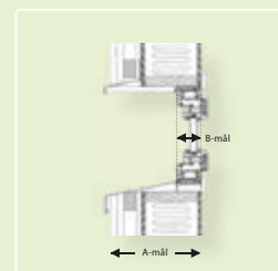
Innvendig montering.
